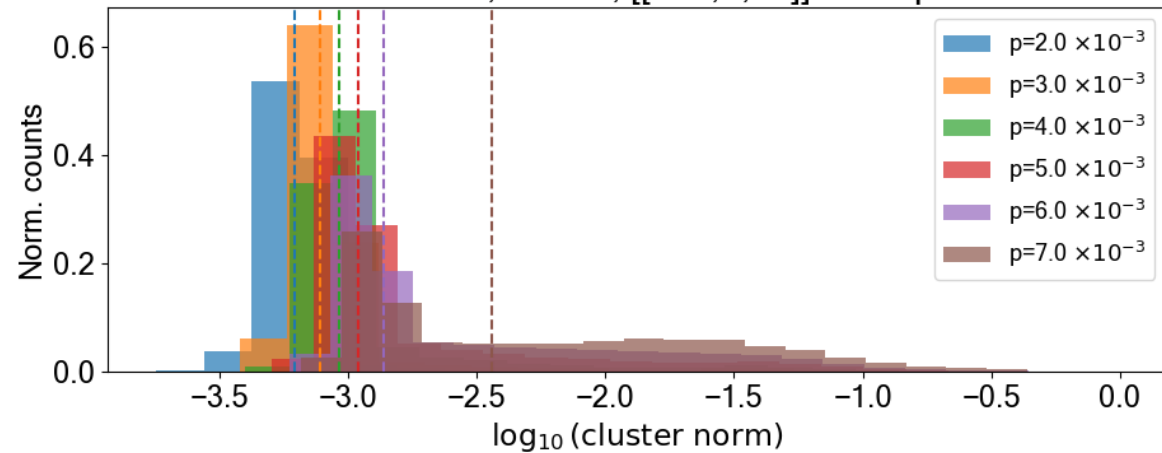
N = 100000, r = 25, [[162, 8, 14]] with bplsd
